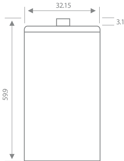
Typical dimensions (mm). Without tube.
